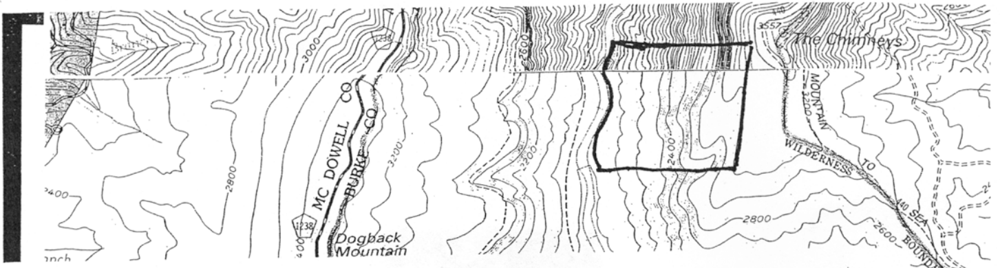
Ashford & Linville Falls Quad Maps
